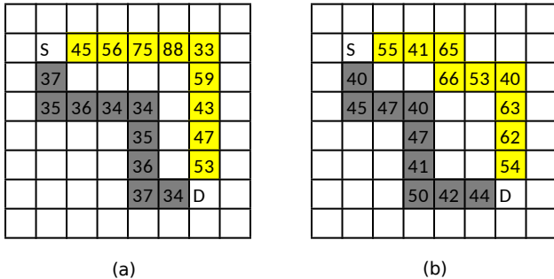
Figure 4: Numerical values refer to RUL(b) . In (a) the dark left path is better according to the minimum RUL value (34 against 33), but when using this path many worn blocks become even more worn. In (b) the two paths are equal according to the minimum RUL value (40), but the light right path is better since its blocks have generally higher values.
